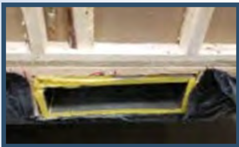
Fiberglass Heat Ducts w/in Floor Cross Over Heat— Standard
